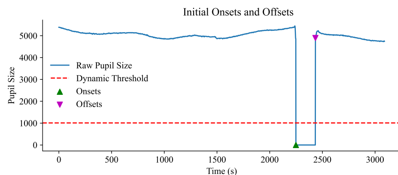
Fig. 5 Initial detection of blink onsets and offsets. These preliminary values may be further refined in subsequent steps to improve accuracy
