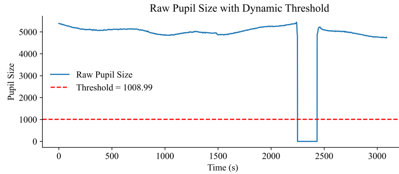
Fig. 3 Dynamic thresholding establishes an adaptive threshold for detecting blink events based on pupil size distribution
